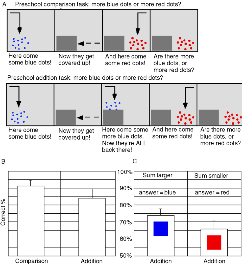
Fig. 3. Preschool comparison and addition. (A) Task schematic. (B) Comparison and addition data, with 95% confidence intervals. Performance in both conditions is >chance (both t(16) > 12 , P < 0.0001 ). Comparison performance was better than addition (matched sample t(16) = 2.73 , P < 0.05 ). (C) Addition performance by 5-year-olds in a second experiment, plotted separately for sum-larger and sum-smaller problems, reveal above-chance performance in both conditions ( t(17) = 4.64 , P < 0.0003 for sum-larger, t(17) = 2.95 , P < 0.01 for sum-smaller). Because both addends were always smaller than the comparison array, success on sum-larger problems required genuine approximate addition.
